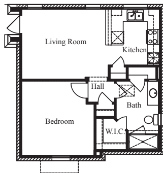
Casita Layout 2 at Front 1 Car Garage
