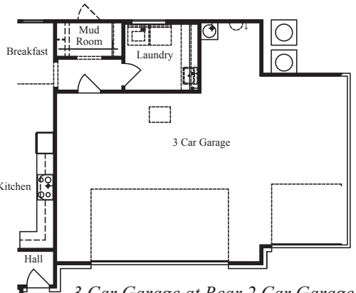
3 Car Garage at Rear 2 Car Garage
