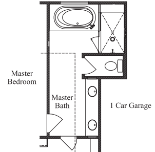
39" x 71" Drop-In Tub with Mudset Shower at Master Bath
