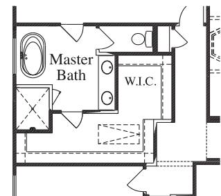
Stand-Alone Tub with Mudset Shower at Master Bath
