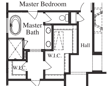
Stand-Alone Tub with Mudset Shower at Master Bath
