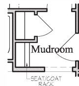
Bench with Coat Hooks at Mudroom
