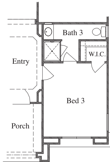
Flip Bed 3/Bath 3 Layout
